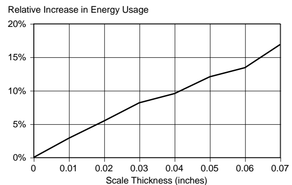
Figure 3. Scale Impact on Energy Usage
